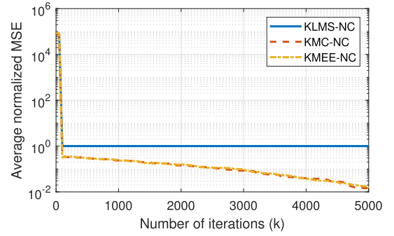
(a) Average normalized MSE
