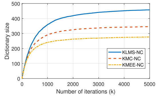
(b) Dictionary size
