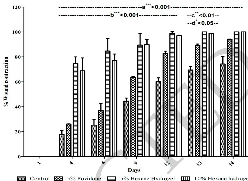
Figure 3. Potential of various n-hexane extract of M. oleifera seeds hydrogels on the healing of excision wound expressed in percentage. Mean \pm SD, analyzed by Two- way ANOVA (Analysis of variance) followed by Bonferroni's multiple comparison test post hoc analysis; a*** < 0.001 vs. control; b*** < 0.001 test drugs vs. standard until 12th day; c** < 0.01 5% hexane hydrogel vs. standard at 13th day; d* < 0.05 10% hexane hydrogel vs. standard at 13th day.
